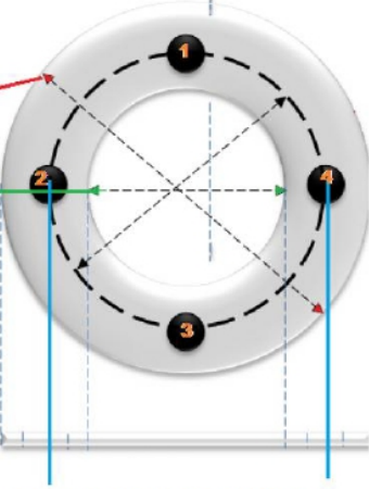
PCD - PITCH CIRCLE DIAMETER MEASURED AS THE DISTANCE FROM THE CENTRE OF ONE BOLT HOLE TO THE CENTRE OF THE BOLT HOLE OPPOSITE THROUGH THE IMAGINARY CENTRE POINT OF THE GASKET
