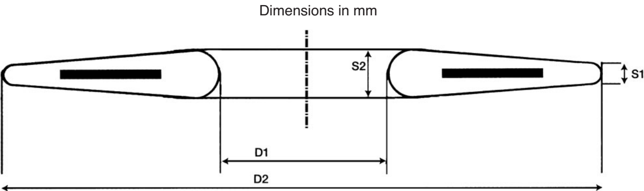
Example for gasket dimensions type G-SS-Standard
