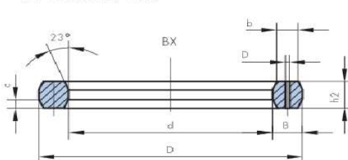
STYLE M19-BX
