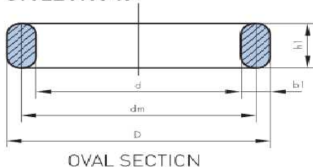
STYLE M19-BX
