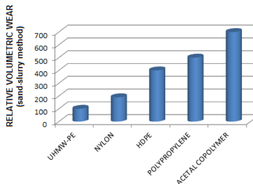
ABRASION RESISTANCE
