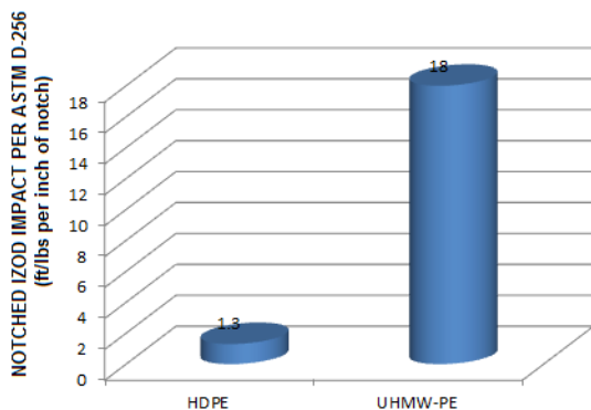
IMPACT RESISTANCE
